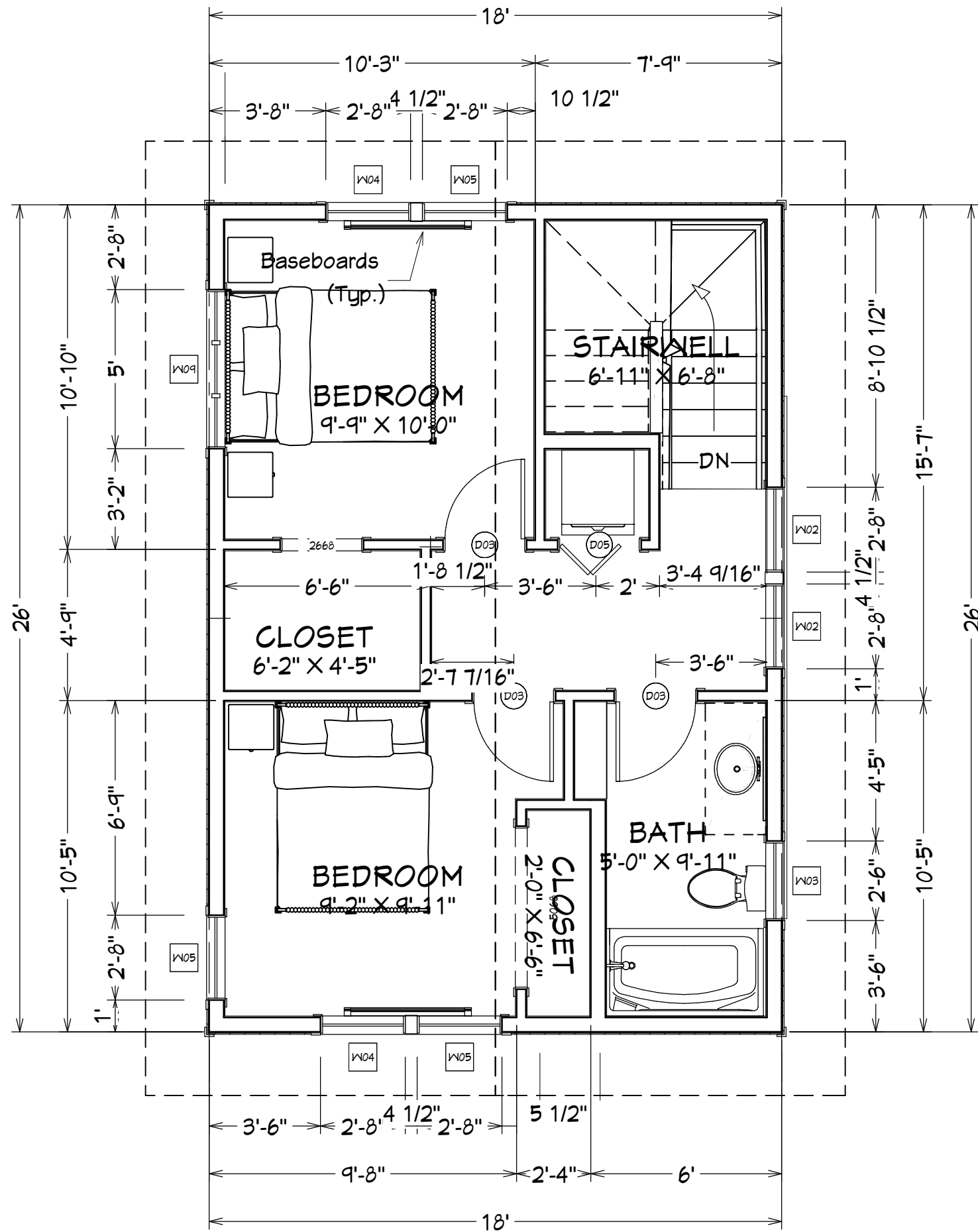
2nd Floor 1/4 in = 1 ft
